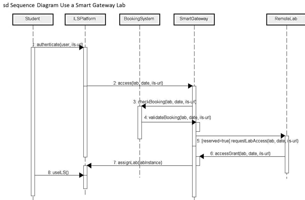
Figure 23. A sequence diagram that models how a booked remote lab hosted on the Smart Gateway is used in an ILS.
