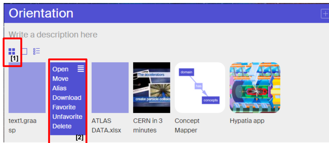
Figure 35: Thumbnail view
