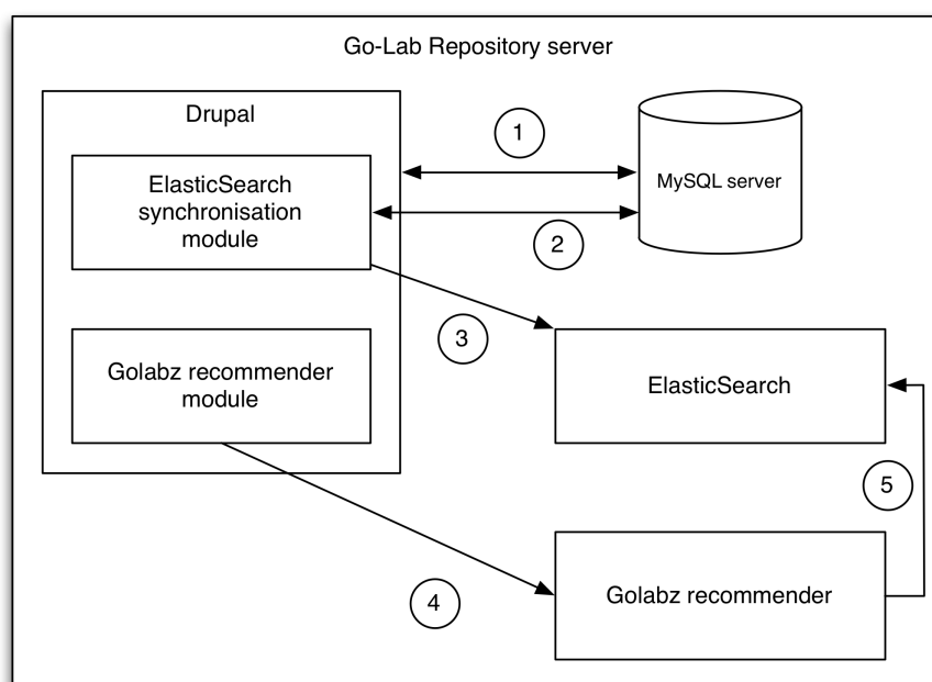
Figure 16. Architecture of the Go-Lab recommender system.
