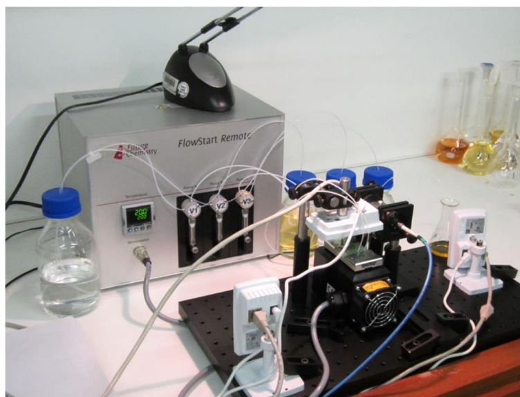
Figure 2 The "Methyl orange" remote lab (photo reprinted with permission) c .
