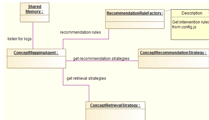
Figure 13. Components related to the Concept Mapping Agent
