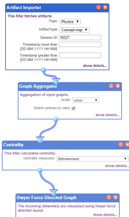
Figure 8. Workflow for concept map aggregation.
