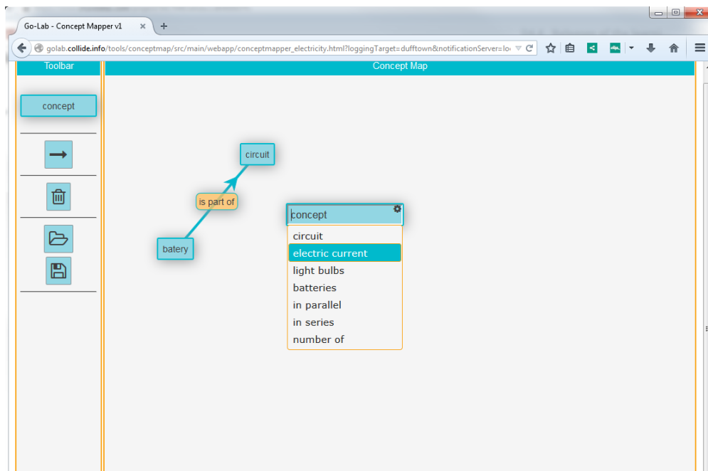
Figure 14. Recommendation of concept lists.
