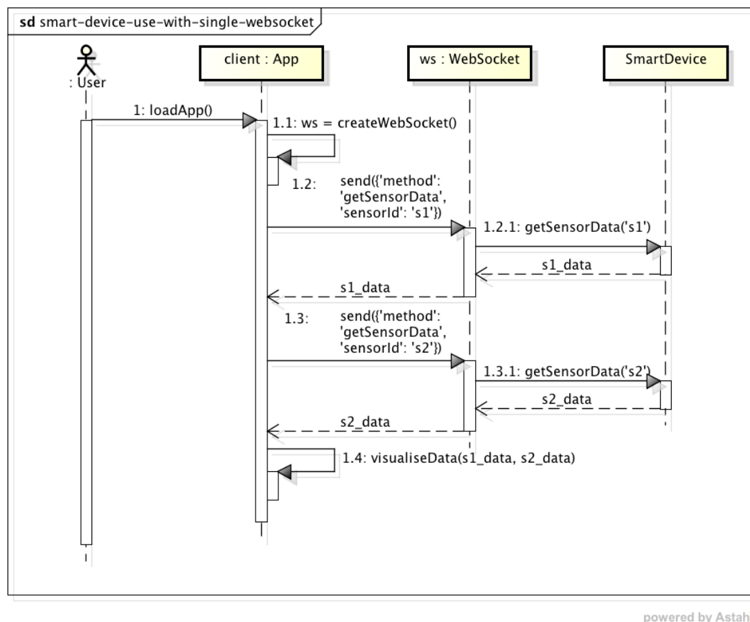
Figure 12: UML Sequence diagram on the use of a single WebSocket for connecting to multiple Smart Device services.
