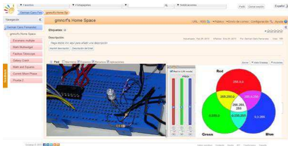
Figure 4. The RGB LED lab integrated in an inquiry learning space. The various Web apps connect to the specified services (video stream, actuators).
