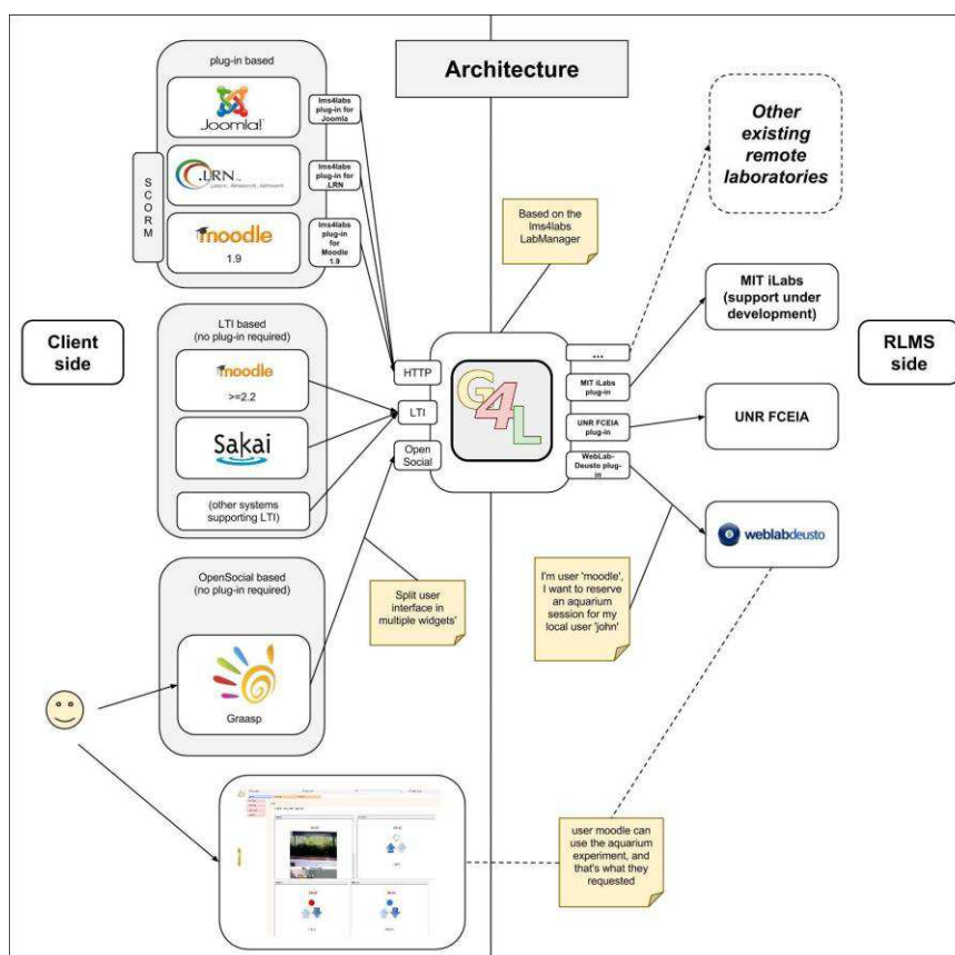
Figure 13. G4Labs architecture.
