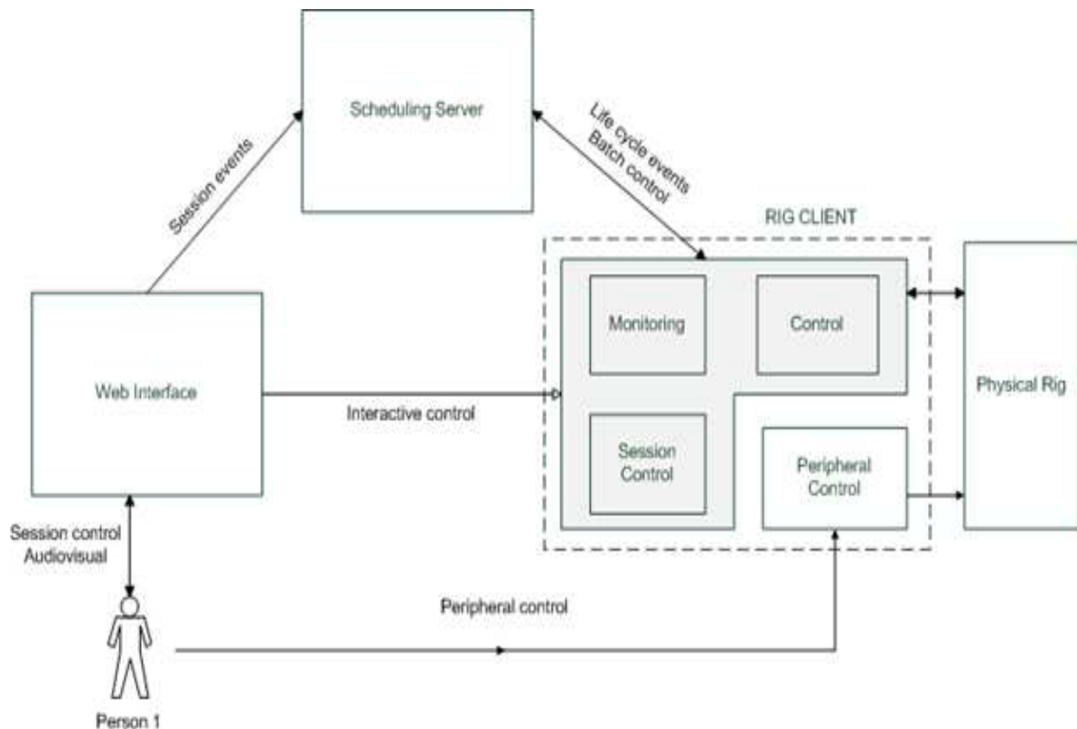
Figure 14. Sahara architecture.
