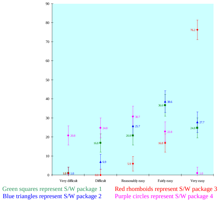
Figure 1: Ease of Use
