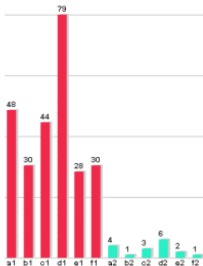
Figure 1: Histogram of mean response time in seconds (bars a1..f1) and number of errors (bars a2..f2) across the different interaction styles: (a) command language, (b) pop-up menus, (c) pull- down menus, (d) forms, (e) direct manipulation by click, (f) direct manipulation by drag & drop
