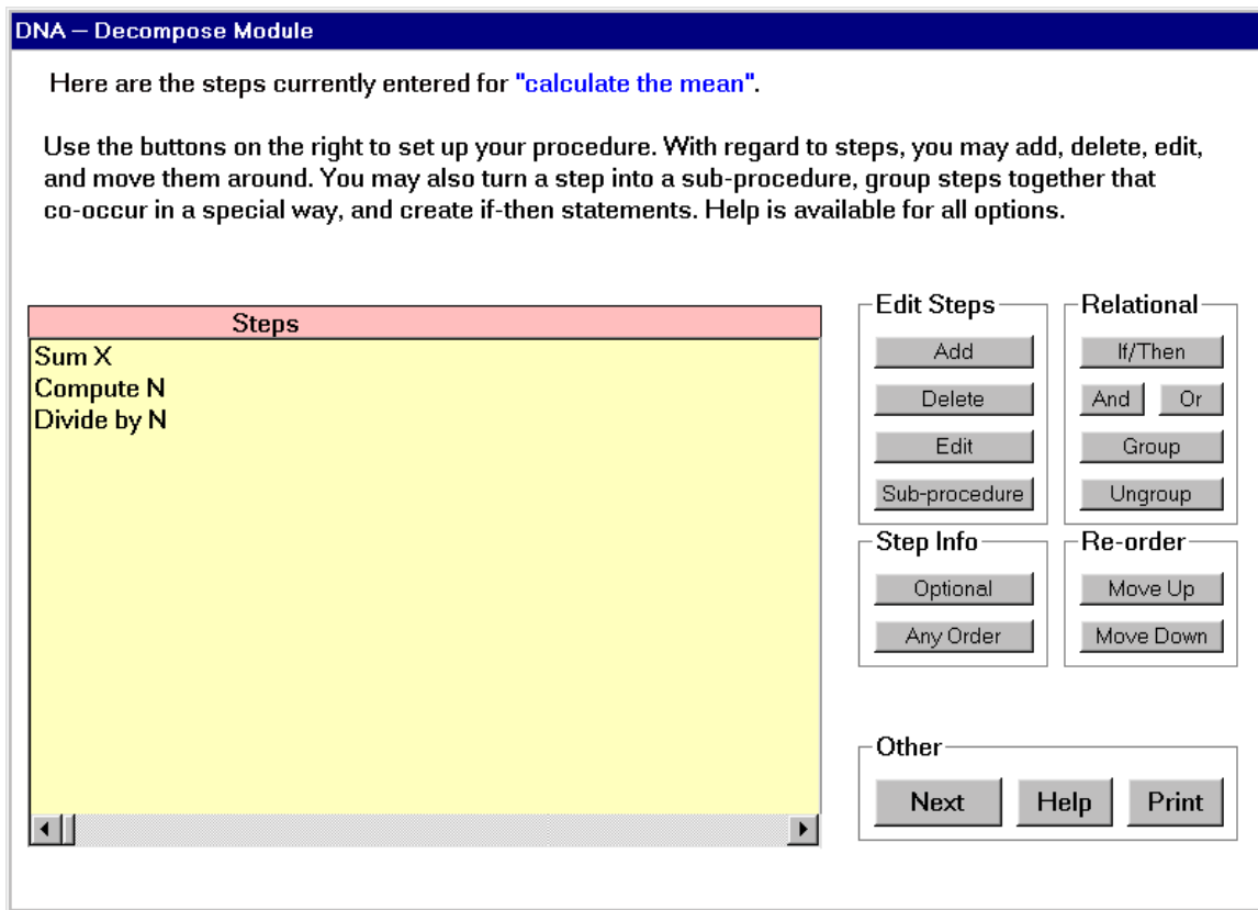
Figure 3. An example of the step-editor screen, from the procedural knowledge (PK) path, with the steps for calculating the mean.
