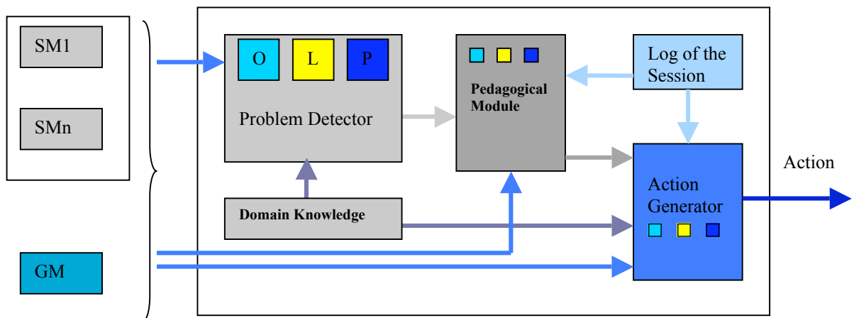
Fig. 2. SSMB architecture showing flows of information.
