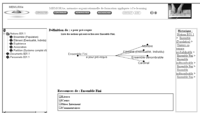
Figure 2: Horizontal navigation
