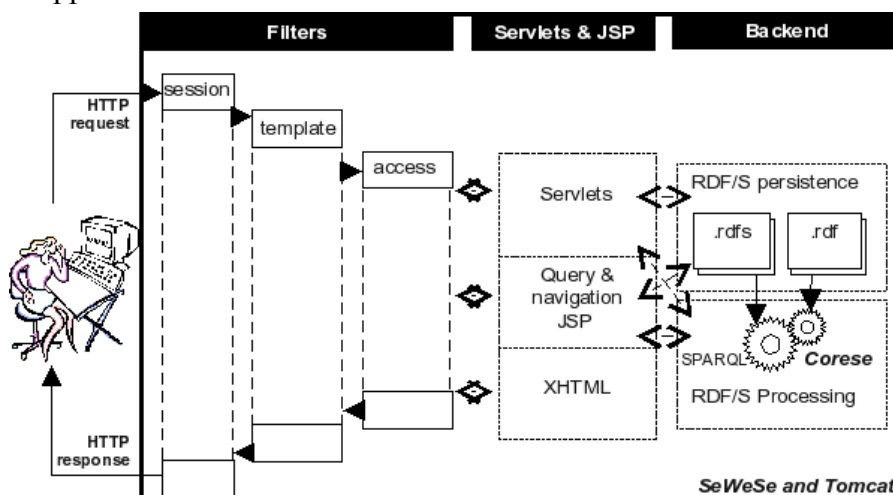
Figure 9.1: SeWeSe architecture
