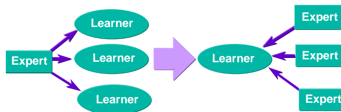
Figure 1 - Paradigm shift
