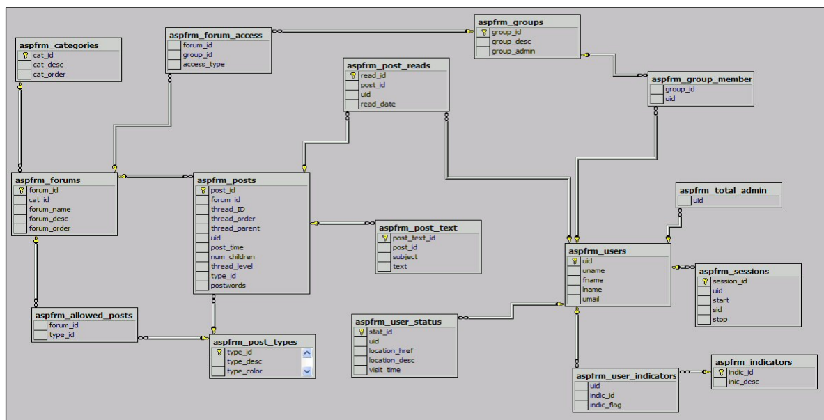
Figure 2: Database Schema
