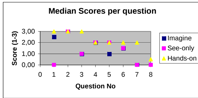
Figure 5-4: Performance per question based on median scores
