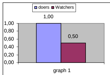
Figure 7-2: Performance in the first question (graph 1), in median scores
