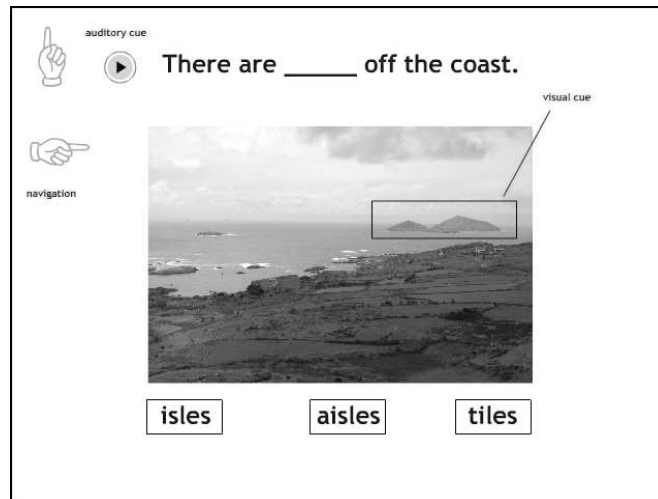
Figure 19: Fill-in Interaction
