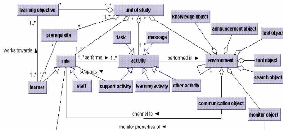
Figure 2.3 Le Unit of Study Model de EML
