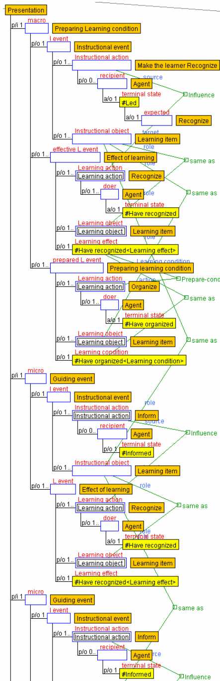
Figure 15 Definition of “Presentation” WAY-knowledge (a portion)
