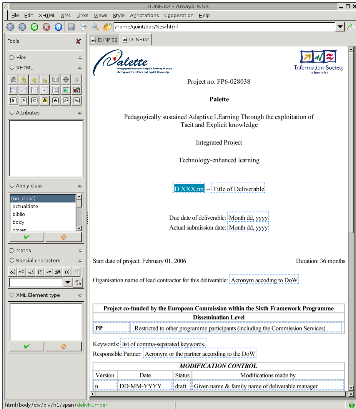
Fig. 2: A new document created from a template
